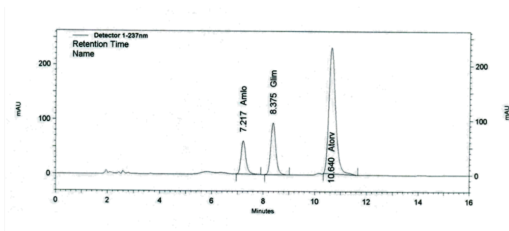
Figure 3.5. The resolution pattern of amlodipine, glimepiride and atorvastatin mixture dissolved in diluent and plasma respectively.
